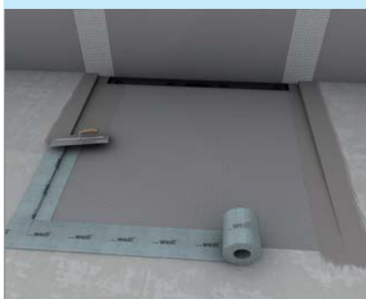
... seal, level ...
