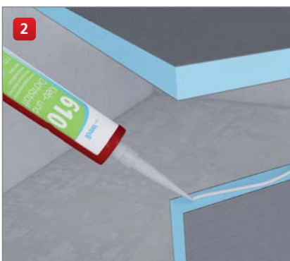
... assemble elements with wedi 610 ...
